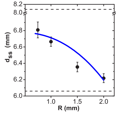
FIG. 4. (Color online) Distance d_{ss} of the stationary filament from the opposite bead as a function of the radius R of the pinning beads. The distance is measured along the central symmetry line of the equilateral bead triangle. The two dashed lines are the geometric limits of a circular (top) and triangular (bottom) filament. With respect to the three bead centers, they equal the diameter of the circumcircle and the height of the bead triangle, respectively. The continuous curve is the best fit of Eq. (7) to the experimental data. The bead distance is kept constant at 7 mm.
