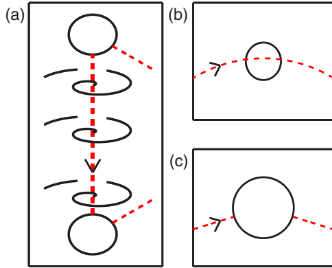
FIG. 1. (Color online) Schematics of a filament (dashed, red line) pinned to two inert spheres (a). The smaller panels show the limiting cases of a locally pinned, smooth filament (b) and a filament cut into two independent segments (c).
