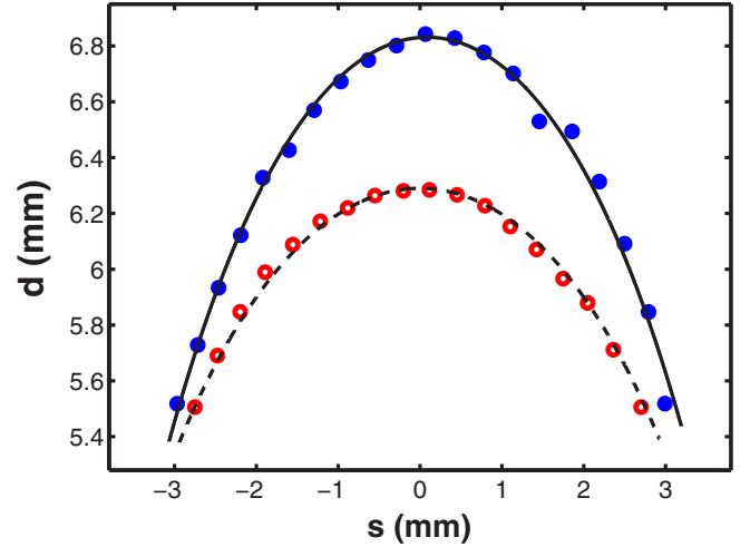
FIG. 6. (Color online) Averaged shape of the stationary filament for R = 0.75 mm (open, red circles) and 1.5 mm (solid, blue circles). The dashed and solid curves represent the corresponding hyperbolic cosine fits [Eq. (3)] which allow the measurement of the filament rigidity \epsilon (see Table I). For both experiments the bead distance is \Delta = 7 mm.
