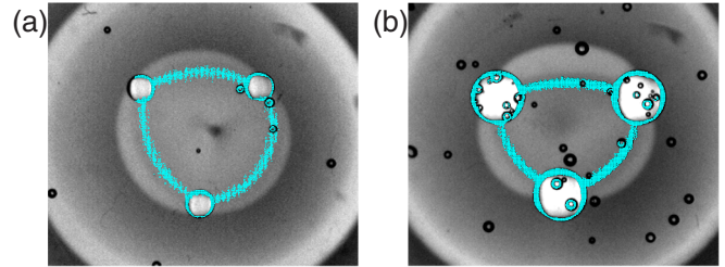
FIG. 2. (Color online) Top view of scroll rings in 1 cm thick layers of BZ reagent. The superposed filaments (bright, cyan) are pinned to three beads (white) of radius (a) 0.75 mm and (b) 1.5 mm. The filaments are stationary and slightly more curved in (a) than in (b). The center-to-center bead distance and image area are 7 mm and (16.5 \times 14) mm 2 , respectively. The images are obtained 120 min after the start of the reaction and show some CO 2 bubbles (dark spots).
