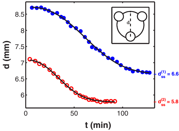
FIG. 3. (Color online) Relaxation dynamics of the pinned filament into the stationary state. The distance d is measured from one bead center to the midpoint of the filament fragment opposite to it. This distance is shown schematically in the inset (dashed line). The experimental data sets are obtained for a bead distance of 6 mm (open, red circles) and 7 mm (solid, blue circles). The bead radius in both cases is 1 mm. Solid curves represent best-fit compressed exponentials.
