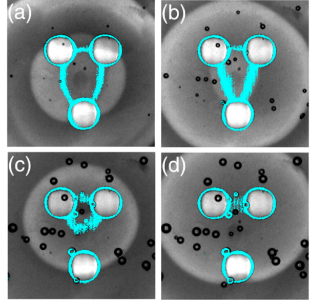
FIG. 7. (Color online) Still frames illustrating the evolution of a filament pinned to three beads located on an isosceles triangle. The snapshots are taken at t = 27 min (a), 67 min (b), 123 min (c), and 140 min (d). The filament unpins at the tight angle and collapses.
