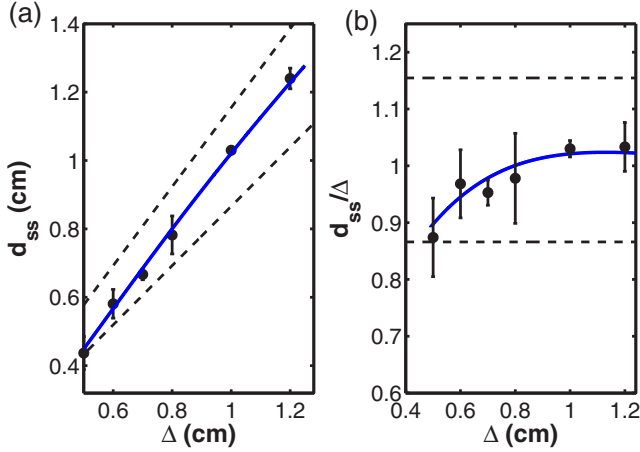
FIG. 5. (Color online) Distance d_{ss} of the stationary filament from the opposite bead as a function of the bead distance \Delta (a). In (b) the same data are shown in terms of the ratio d_{ss}/\Delta . As in Fig. 4, the dashed lines correspond to the geometric limits of a circular (top) and triangular (bottom) filament. The continuous curves are the best fit of Eq. (7) to the experimental data. The bead radius is kept constant at 1.0 mm.
