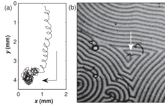
FIG. 11. Defect dynamics under the influence of three forcing wave patterns. (a) Trajectory of the spiral defect. (b) Superposition of three snapshots obtained from the same experiment after the defect reached its final position. The time between each snapshot corresponds to one third of the forcing period. The arrow in (b) indicates the final position of the defect. Field of view 7.0 \times 7.9 mm 2 . The experiments were carried out for reactant concentrations described by set II.
