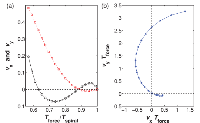
FIG. 2. (Color online) Spiral defect motion in planar wave trains computed from numerical simulations. (a) Velocity components v_x (black circles) and v_y (red squares) as a function of the ratio between the periods of the forcing wave train T_{\text{force}} and the unperturbed spiral T_{\text{spiral}} . The forcing waves travel in +y direction. The defects rotate counterclockwise. (b) Shift in defect position per forcing period obtained from the same data by graphing v_y T_{\text{force}} vs v_x T_{\text{force}} . Notice that drift into three different quadrants is observed.
