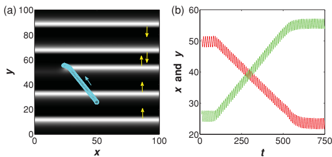
FIG. 3. (Color online) Defect drift in the wave field of two planar wave trains. The defect stops within the collision zone of the planar waves. (a) V-concentration pattern of the halted defect with its superposed (cyan) trajectory. The arrows indicate the direction of wave propagation and defect drift. (b) Time evolution of the x (red/dark gray) and y (green/light gray) coordinates of the defect tip. Forcing period T_{\text{force}} = 9.5 and T_{\text{force}}/T_{\text{free}} = 0.8 .
