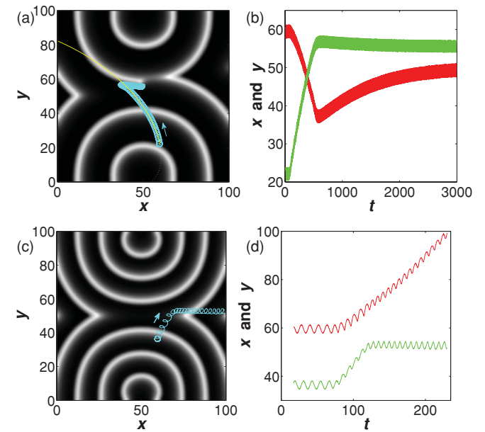
FIG. 4. (Color online) Two representative examples of defect drift in the wave field of two circular wave trains. (a) and (c) V-concentration pattern of the spiral defect with its superposed (cyan) trajectory. The arrows indicate the direction of the defect drift. The smooth (yellow) curve in (a) is a logarithmic spiral. (b) and (d) Corresponding time evolution of the x (red/dark gray) and y (green/light gray) coordinates of the defect tip. The target patterns have frequencies of T_{\text{force}} = 9.5 in (a) and (b) and 7.0 in (c) and (d). Accordingly T_{\text{force}}/T_{\text{spiral}} is 0.8 in (a) and (b) and 0.59 in (c) and (d).
