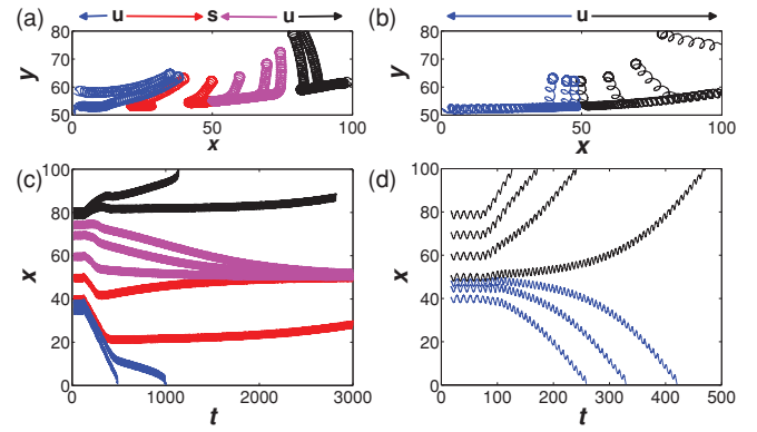
FIG. 5. (Color online) Drift trajectories (a) and (b) and corresponding x coordinates (c) and (d) of spiral defects with different initial positions. The forcing waves are generated by two target patterns analogous to the situation shown in Fig. 4. The wave periods of the target patterns are T_{\text{force}} = 9.5 in (a) and (c) and 7.0 in (b) and (d). For the lower period the system shows one stable attractor “s” at x = 50 and two repellers “u” at approximately x = 20 and 80 . For the higher period, the central point is a repeller. Left and rightward diverging trajectories are plotted in blue and black (darker lines in grayscale), respectively, while attractor-bound curves are shown in red and magenta (lighter lines in grayscale).
