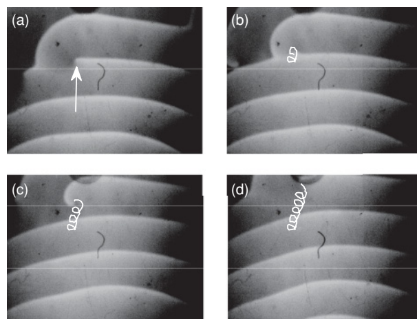
FIG. 7. Defect drift in a thin layer of the Belousov-Zhabotinsky system. The time between subsequent snapshots is 940 s. The forcing waves travel in upward direction. The frequency ratio between the forcing waves and the unperturbed spiral wave is 0.57. The defect drifts toward the upper right corner tracing the white trajectories superposed on frames (b)-(d). The white arrow in (a) marks the initial position of the defect. The initial reactant concentrations are listed in the text as set I. The field of view is 2.44 \times 1.83 cm ^2 .
