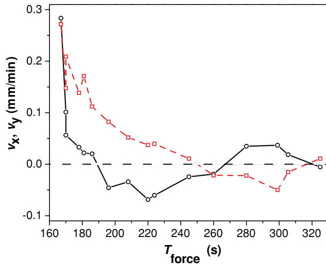
FIG. 8. (Color online) Drift velocity of spiral defects in single, near-planar wave trains as a function of the forcing period. The values of v_x (black open circles) describe the velocity component along the forcing wave fronts, while v_y (red squares) is the velocity component perpendicular to the forcing waves. The experiments were carried out for reactant concentrations described by set I.
