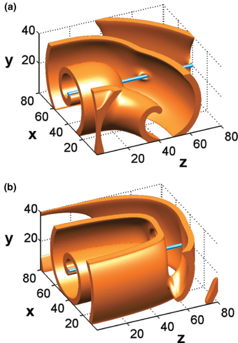
FIG. 4. (Color online) Snapshots illustrating the evolution of a self-wrapping scroll wave. Solid (orange) regions are in an excited state which corresponds to high values of the activator variable u . The unexcitable cylinder (cyan) extends in z -direction and has a radius of 1.0. Notice the increasing length of the pinned scroll wave. The time elapsed between frames is 205 time units, which corresponds to approximately 23 rotation periods.
