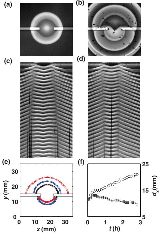
FIG. 3. (Color online) (a), (b) View through a three-dimensional BZ system in which a scroll wave is pinned to two glass cylinders with an individual length of 14 mm and a radius of 1 mm. Frame (a) has been recorded immediately after the initiation of the scroll wave, frame (b) 116 min later. Image area: 32 \times 32 \text{ mm}^2 . (c), (d) Time-space plots constructed along vertical lines slightly above (c) and below (d) the cylinders shown in (a), (b). Time evolves in downward direction and spans 3 h. (e) Reconstructed filaments at 16 min (black triangles), 76 min (blue squares), and 256 min (red circles). (f) Temporal evolution of the width of the upper (circles) and lower (squares) filament arches.
