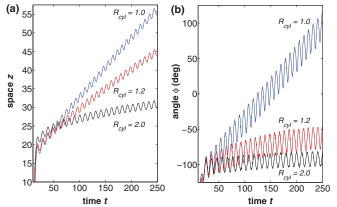
FIG. 5. (Color online) Filament movement along the pinning cylinder for cylinder radii of 1.0 (blue), 1.2 (red), and 2.0 (black). The time traces describe the motion of the end point of the free filament near the pinning cylinder. Using cylindrical coordinates (r, \phi, z) , (a) illustrates motion along the cylinder axis and (b) characterizes rotation around the cylinder. In all three cases, the extent of pinning increases over time.
