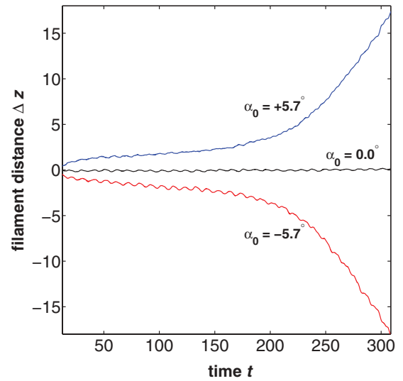
FIG. 9. (Color online) Temporal evolution of the distance \Delta z between the two contact points of the filaments in Fig. 8. From top to bottom the curves correspond to the initial conditions in Fig. 8(a) (blue), 8(b) (black), and 8(c) (red). The contact points are defined as the locations on the filament that have a distance of 2.0 to the surface of the pinning cylinder.
