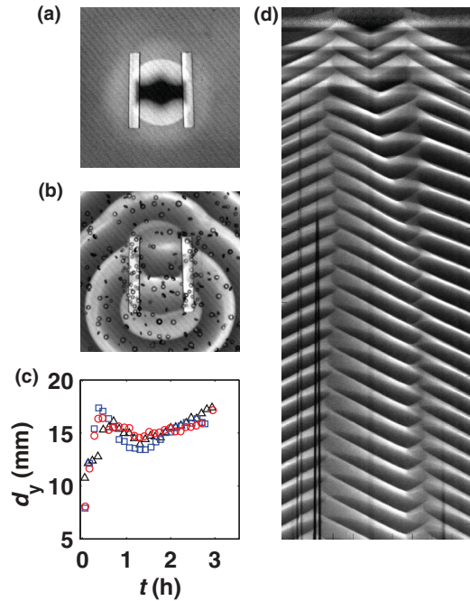
FIG. 2. (Color online) (a), (b) View through a three-dimensional BZ system in which a scroll wave is pinned to two glass cylinders with an individual length of 14 mm and a radius of 1 mm. Frame (a) has been recorded immediately after the initiation of the scroll wave, frame (b) 174 min later. Image area: 30 \times 30 mm 2 . (c) Distance between the upper and the lower filament segments as a function of time. The distance is measured close to the right edge of the left cylinder (red circles), close to the left edge of the right cylinder (blue squares), and in their middle (black triangles). (d) Time-space plot constructed along the vertical line in (a), (b) that has equal distance to the two cylinders. Time evolves in downward direction and spans 3 h.
