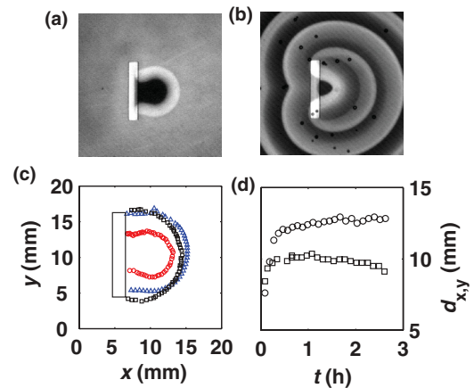
FIG. 1. (Color online) (a), (b) View through a 8 mm thick BZ system in which a scroll wave (grayish pattern) is pinned to a glass cylinder (bright rectangle; height 12 mm; radius 1 mm). Frame (a) has been recorded immediately after the initiation of the scroll wave, frame (b) 116 min later. Image area: 29 \times 29 mm 2 . (c) Filament positions in the same experiment approximately 0 min (red, innermost curve), 8 min (blue triangles), and 196 min (black squares) after initiation. (d) Temporal evolution of the maximal distance d_x between the filament and the cylinder (squares) and the maximal extension d_y of the filament along the cylinder axis (circles).
