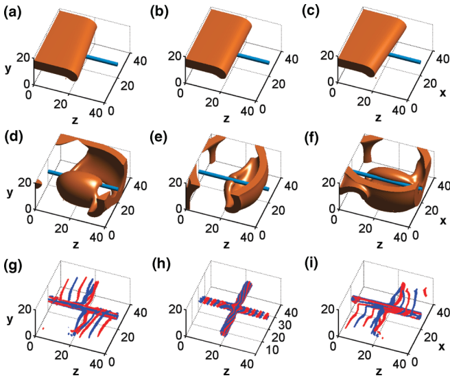
FIG. 8. (Color online) Simulated vortex dynamics for three similar initial conditions. The early filaments are nearly straight lines tilted +5.7^\circ (a), (d), (g), 0.0^\circ (b), (e), (h), and -5.7^\circ (c), (f), (i) away from a line perpendicular to the pinning cylinder. The upper row shows the u pattern shortly after initiation. Solid orange areas are excited and the pinning cylinder (cyan) extends in z direction. The middle row gives the resulting wave patterns approximately 300 time units later. Notice the different rotation directions of the pinned scroll waves in (d) and (f). The corresponding filament motion is illustrated in the bottom row using alternating colors (blue and red) to help distinguish subsequent data sets.
