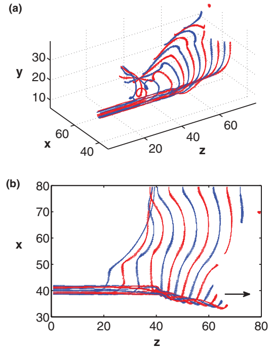
FIG. 7. (Color online) Filament movement along a pinning cylinder (not shown) of radius 1.0. The cylinder length equals only half the system length ( 0 \leq z \leq 40 ). The black arrow indicates the principal direction of filament motion. The time interval between subsequent filament pairs is 35.5 time units. Alternating red and blue colors are used as a visual aid.
