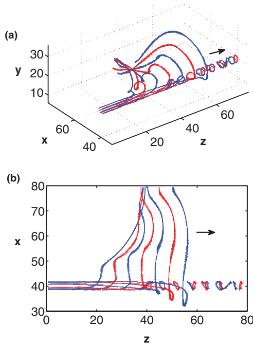
FIG. 6. (Color online) Filament evolution for the partially pinned scroll wave shown in Fig. 4(a) Three-dimensional data; (b) projection into the (x, z) -plane. The pinning, unexcitable cylinder ( R = 1.0 , not shown) extends in z -direction. The black arrows indicate the principal direction of filament motion. The time interval between subsequent filament pairs is 35.5 time units. Alternating red and blue colors are used as a visual aid.
