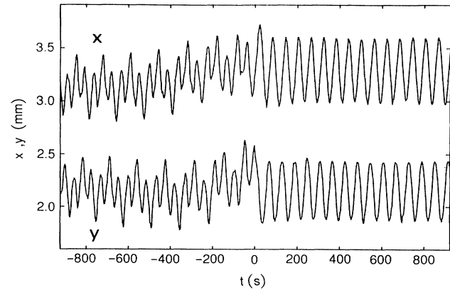
FIG. 2. x and y coordinates of the spiral tip as a function of time. Each curve is composed of 670 values, corresponding to a sample interval of 2.76 s. Up to t = 0 s the tip is meandering and traversing the flowerlike path shown in Fig. 1(a). At t = 0 s the laser is switched on and the resulting unexcitable laser spot region anchors the tip to simple rotation.
