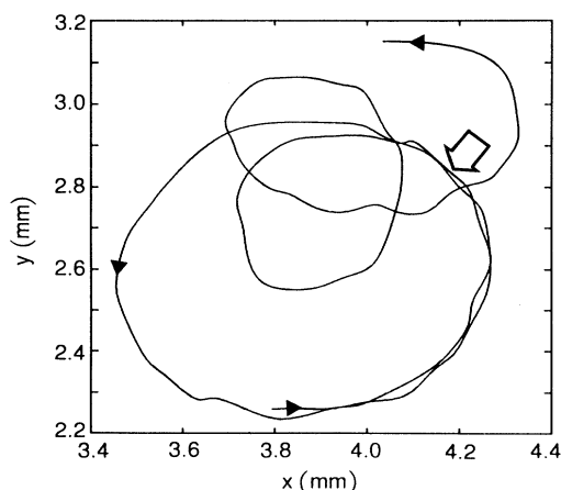
FIG. 4. Anchored spiral tip is released and starts to meander again, when the laser beam is switched off (open arrow). The depicted trajectory of this transition describes a newly formed floral pattern relative to the anchor region. The first loop is located inside the former laser spot area. In this typical experiment the laser was switched on for 240 s. Traversing the depicted path takes the spiral tip 232 s.
