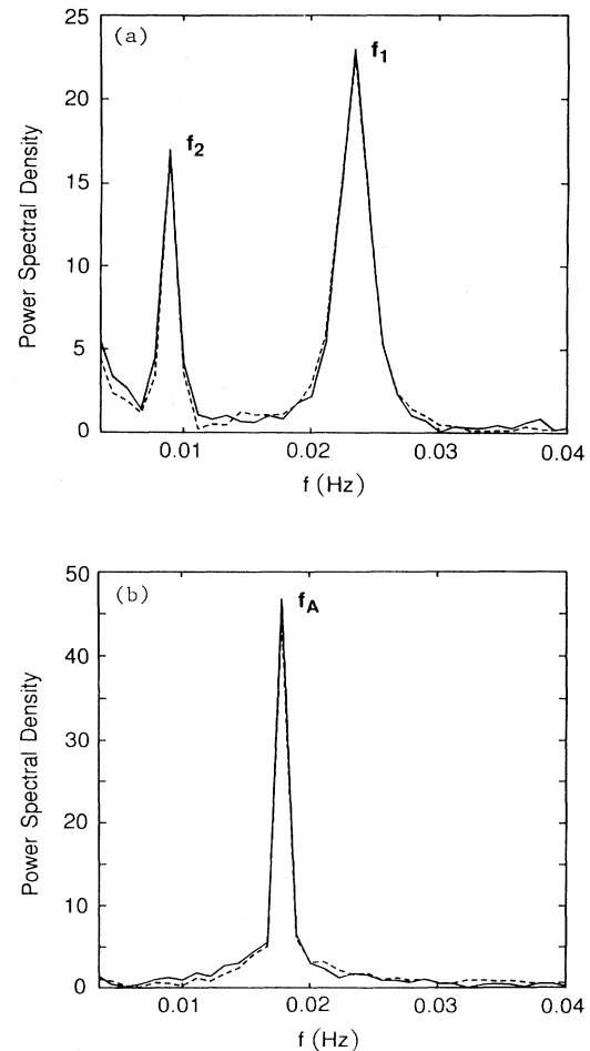
FIG. 3. Power spectra of the data given in Fig. 2: (a) Meandering state ( -925 \text{ s} < t < -31 \text{ s} ), (b) anchored state ( 27 \text{ s} < t < 922 \text{ s} ). Spectrum (a) has two clearly separated peaks at f_1 = 0.0232 Hz and f_2 = 0.0089 Hz, while the anchored tip motion shows only one frequency f_A = 0.0178 Hz. Spectra of x(t) and y(t) are plotted as solid and dashed lines, respectively.
