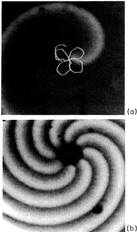
FIG. 1. (a) Digital snapshot of a spiral wave in the ruthenium-catalyzed Belousov-Zhabotinsky reaction observed at 490 nm. The superposed white curve indicates the trace of the unperturbed spiral tip. Image area 2.8 \times 2.8 \text{ mm}^2 . (b) Logical overlay of eight images with a spiral tip anchored by an unexcitable disk (laser spot, diameter 0.4 mm). The tip motion is changed from compound (a) to simple rotation. Time interval between consecutive images: 7.45 s.
