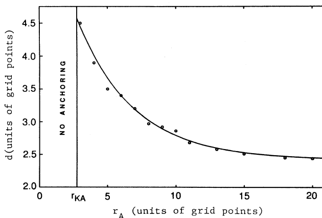
FIG. 6. Distance d between anchor boundary and tip as a function of anchor radius r_A . Resulting from simulations on an array of 256 \times 256 grid points (grid spacing h=0.0863 ) the monotonic decay of d is approximated by an exponential function (solid line). Below a critical value r_{KA} the tip starts again to meander.
