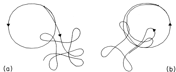
FIG. 5. Simulation of the experimentally observed spiral tip release (Fig. 4) by integration of a simple reaction-diffusion model. The anchor was realized by fixing the values of u (propagator) and v (controller) to (0.0,0.0) in (a) and (0.0,0.5) in (b). The good qualitative agreement between simulation (b) and the experiment can be explained by the production of the inhibitor bromide inside the laser illuminated disk area.
