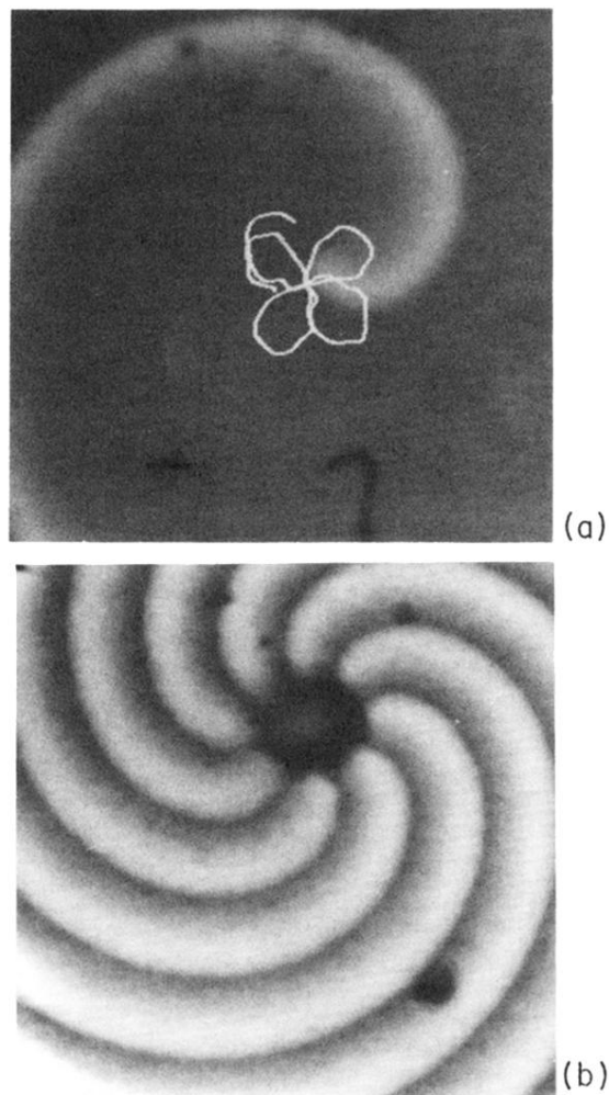
FIG. 1. (a) Digital snapshot of a spiral wave in the ruthenium-catalyzed Belousov-Zhabotinsky reaction observed at 490 nm. The superposed white curve indicates the trace of the unperturbed spiral tip. Image area 2.8 \times 2.8 \text{ mm}^2 . (b) Logical overlay of eight images with a spiral tip anchored by an unexcitable disk (laser spot, diameter 0.4 mm). The tip motion is changed from compound (a) to simple rotation. Time interval between consecutive images: 7.45 s.
